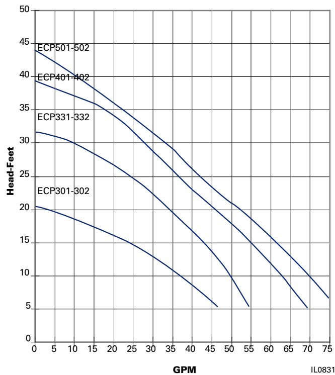
Evaporative Pumps
